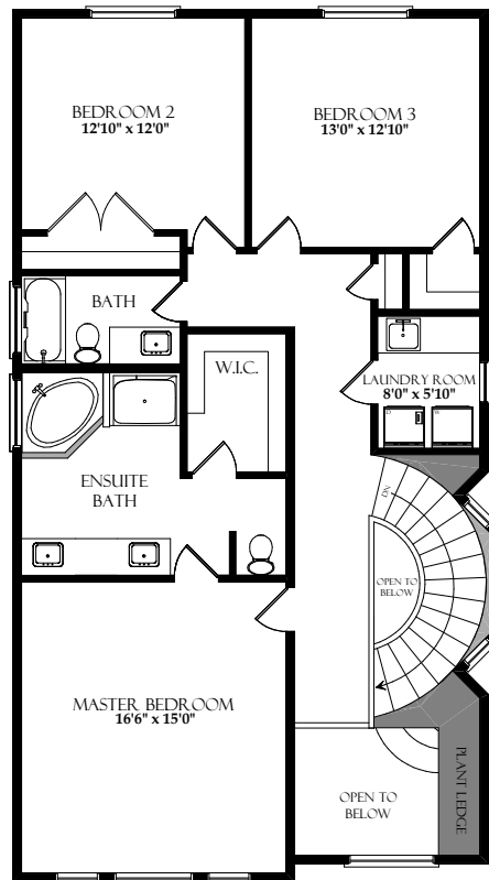
UPPER LEVEL - 1237.99 Sq.Ft.
